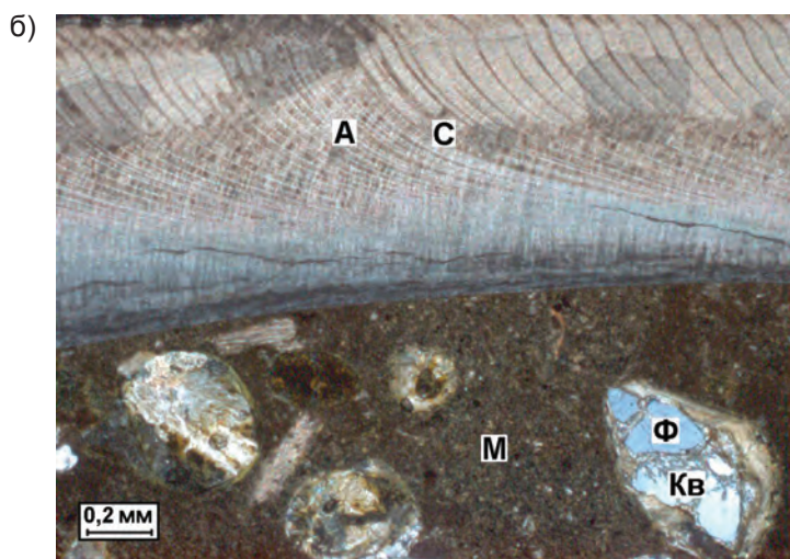
Fig. 3. Polished section (a) and transparent sections (b, c) of productive marl stratum fragment. Nicols X. W—wall of a large aragonite shell; F—fine mineralized fossil shells; M—marl; Q—quartz; S—siderite; C—calcium; A—aragonite
